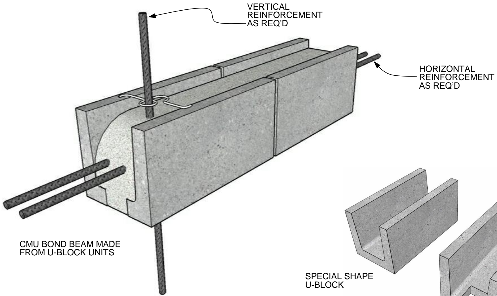
U-BLOCK NOTCHED TO ACCEPT VERTICAL REINFORCEMENT
